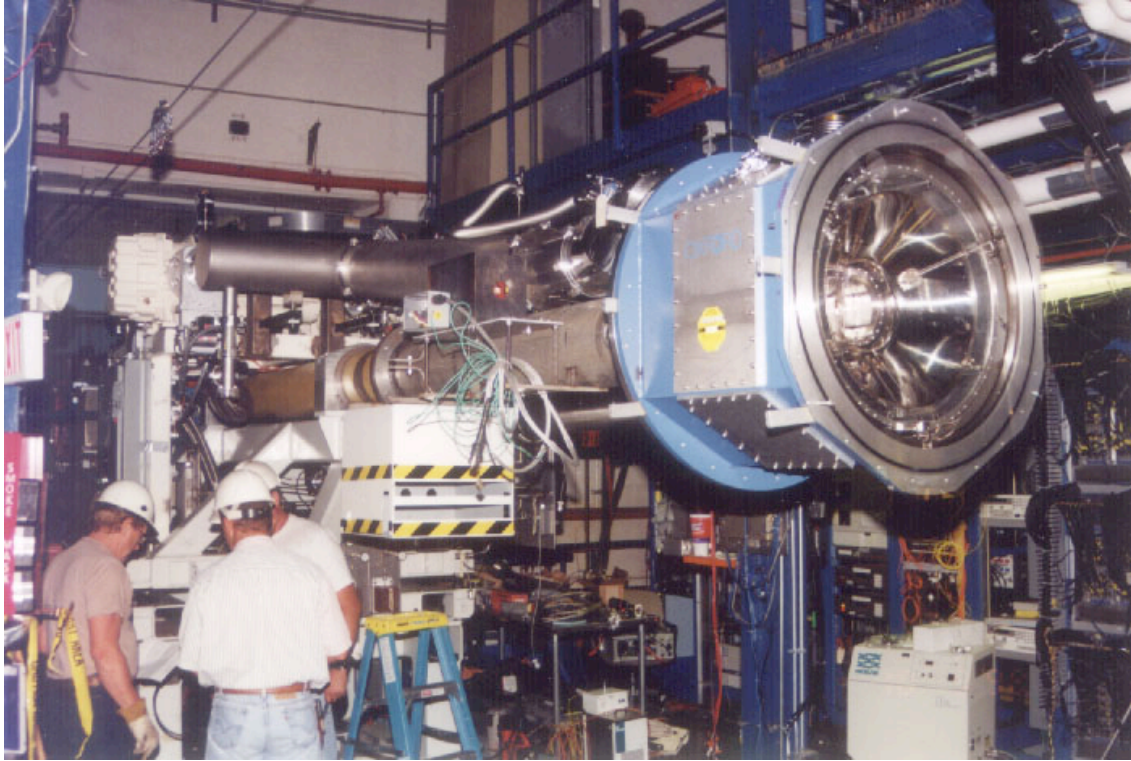
Figure 2: The polarized hydrogen target used for the experiments at Jefferson Lab. The blue vacuum vessel to the right contains a superconducting magnet (50000 Gauss field) and a Helium refrigerator (-272 degrees Celsius, just one degree above absolute zero). The hydrogen nuclei (protons or deuterons) contained in molecules of ammonia ( \text{NH}_3 ) can be polarized under these conditions, using microwave frequency irradiation. The electron beam enters through the large pipe to the left, and the scattered particles are detected in the CLAS spectrometer (outside the picture, to the right).
